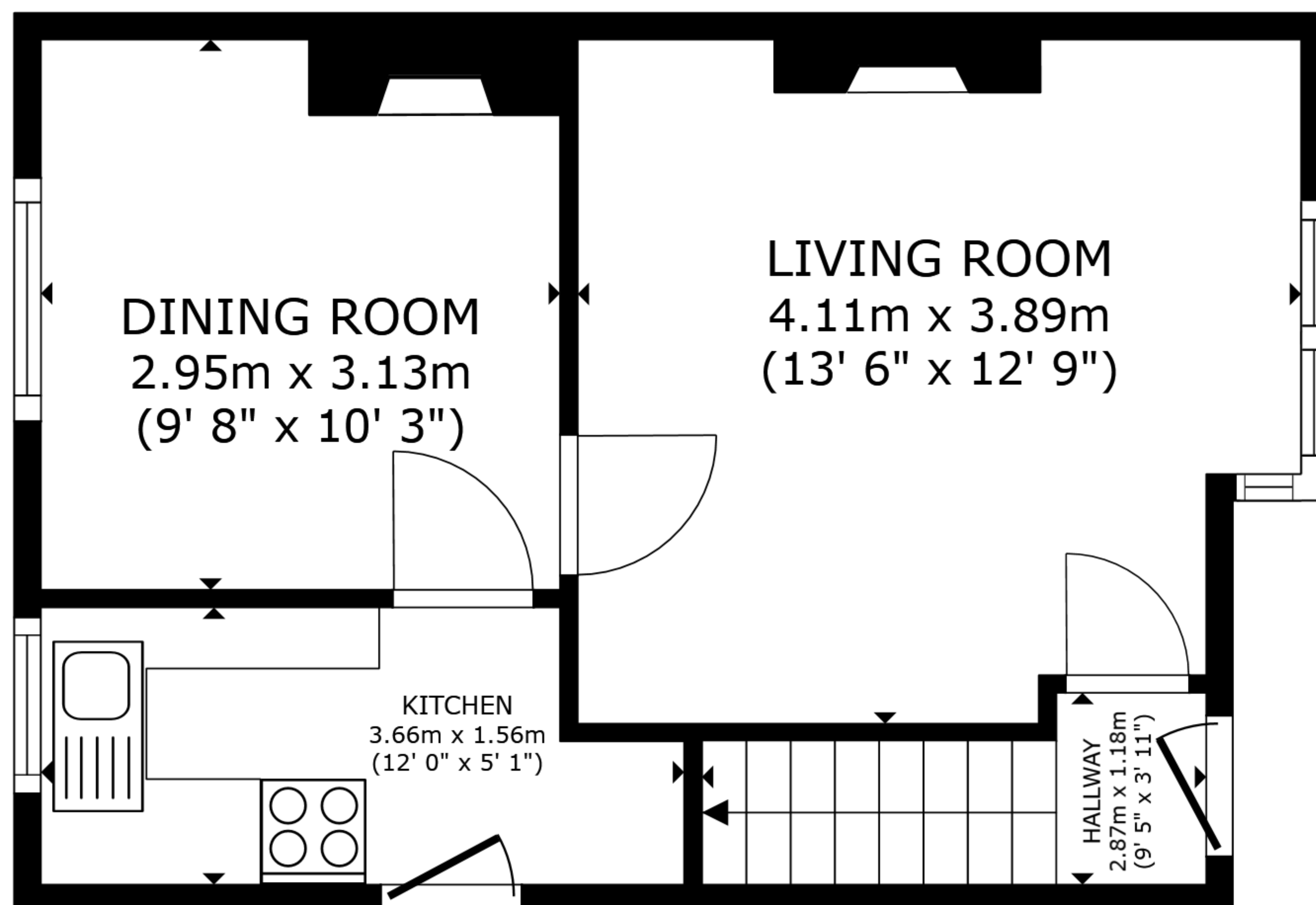
FLOOR 1
