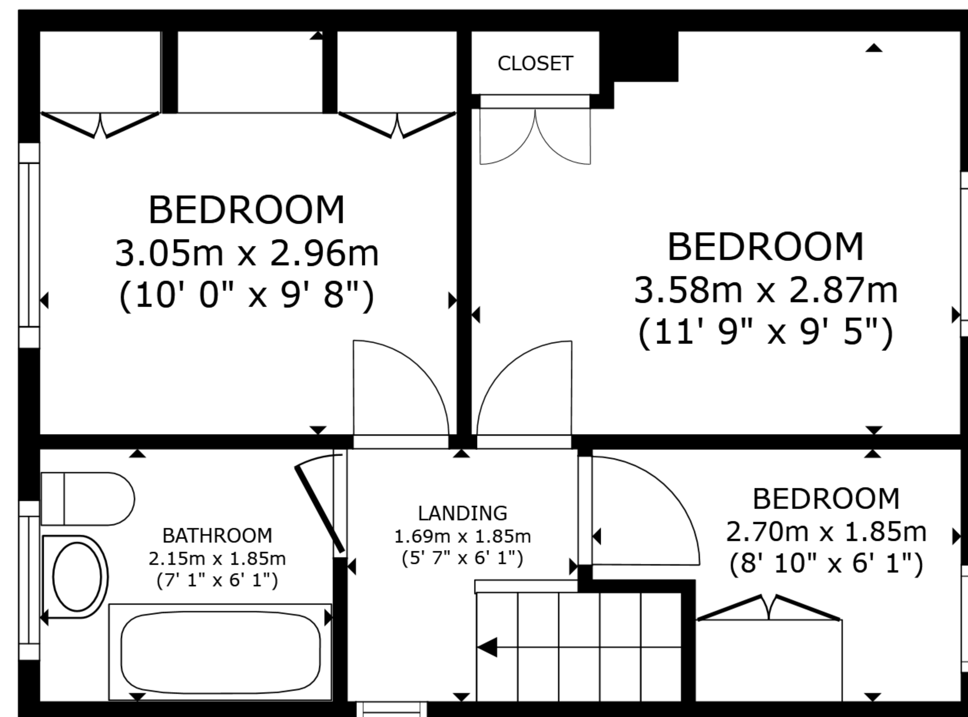
FLOOR 2
